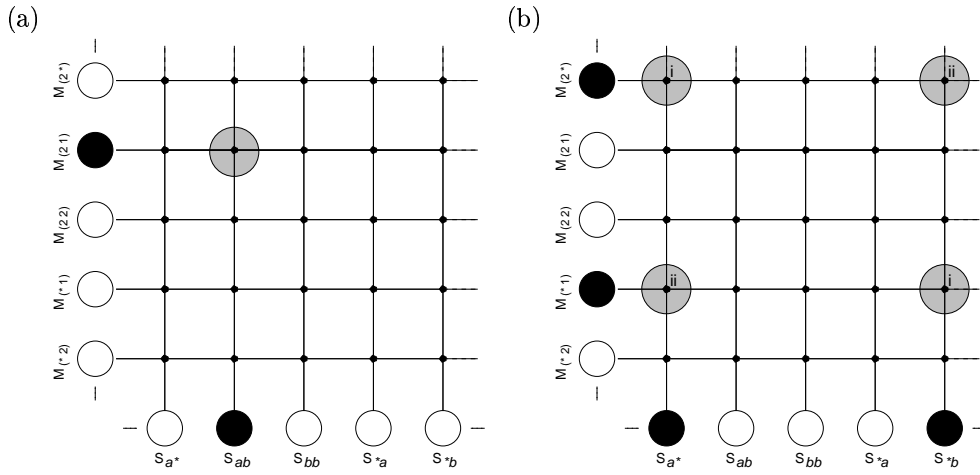
Figure 7: Retrieval of three possible analyses of \langle(2\ 1), ab\rangle . The relevant connection weights are highlighted in grey. (a) g for the one-component analysis \langle\{(2\ 1)\}, \{ab\}\rangle depends on the weight of the connection between the nodes representing the components (2\ 1) and ab . (b) g for the two-component analysis \langle\{(2\ ^*), (^* 1)\}, \{a^*, ^*b\}\rangle depends on the weighted sum of two connections, marked as i. The g for the alternative two-component analysis \langle\{(2\ ^*), (^* 1)\}, \{^*b, a^*\}\rangle is given by the weighted sum of the two connections marked ii.
