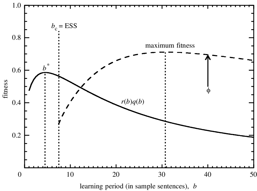
Figure 2. The evolutionary selection of the number of sampling events in the case of a fully symmetrical system. The parameters are as in figure 1 except c_1 = 0.3 and c_2 = 0.1 . The value b^* is below the error threshold, so the ESS is the value b_c .
