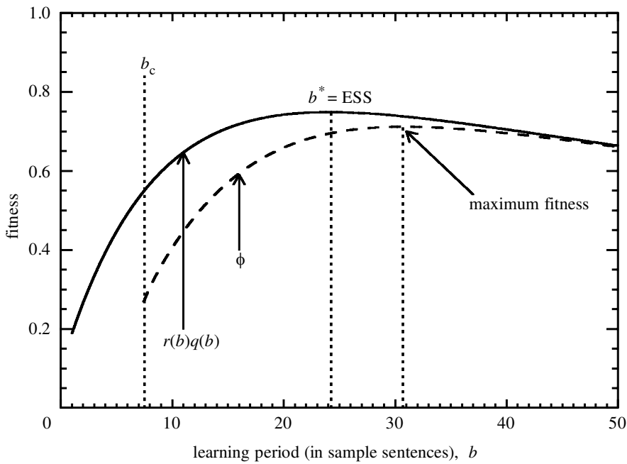
Figure 1. The evolutionary selection of the number of sampling events in the case of a fully symmetrical system; a = 0.5, n = 40, c_1 = 1, c_2 = 0.001 . The value of b which corresponds to the ESS coincides with b^* .
