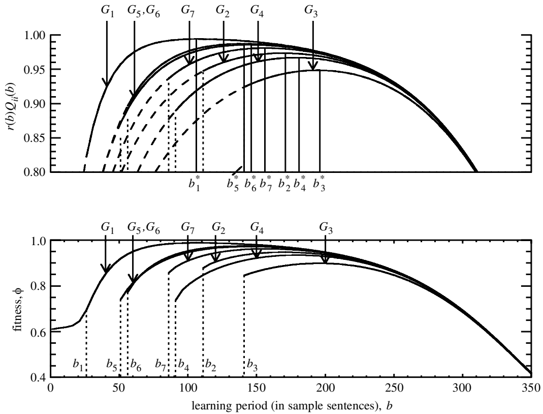
Figure 3. The evolutionary selection of the number of sampling events in the general case; a_{ij} are chosen from a uniform distribution between zero and unity, n = 7 , and r(b) = (c_1 + c_2 \exp(\gamma b))^{-1} with c_1 = 1, c_2 = 0.0005, \gamma = 0.02 . The first plot presents the functions r(b)Q_{ii}(b) , the solid lines correspond to \alpha_i(b) . The second plot shows the average fitness corresponding to one-grammar solutions, for different dominant grammars. Each value b_i denotes the coherence threshold corresponding to the emergence of the one-grammar solution with the dominant grammar G_i . All the values b_i^* in this example correspond to ESS.
