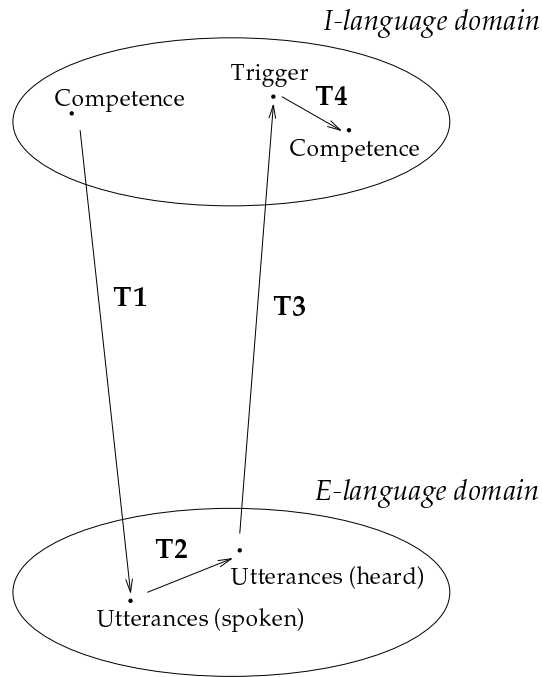
Figure 4: Transformations within and between I- and E-language domains
