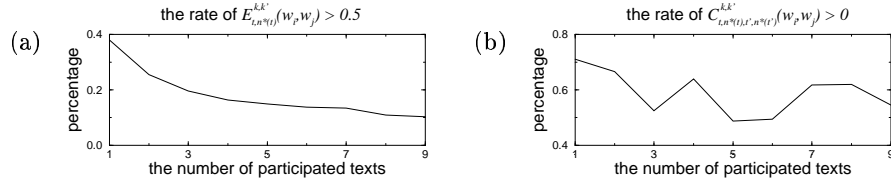
Fig. 7. (a) The ratio of elements for which the difference between two agents larger than 0.5 ( E_{t,n^*(t)}^{k,k'}(w_i, w_j) > 0.5 ) for a pair of agents to all elements in a difference matrix vs. the number of texts in which the pair converses. (b) Transition of the ratio of elements for which the difference between two agents becomes larger ( C_{t,n^*(t),t',n^*(t')}^{k,k'}(w_i, w_j) > 0 ) for a pair of agents to all elements in a change matrix through conversations.
