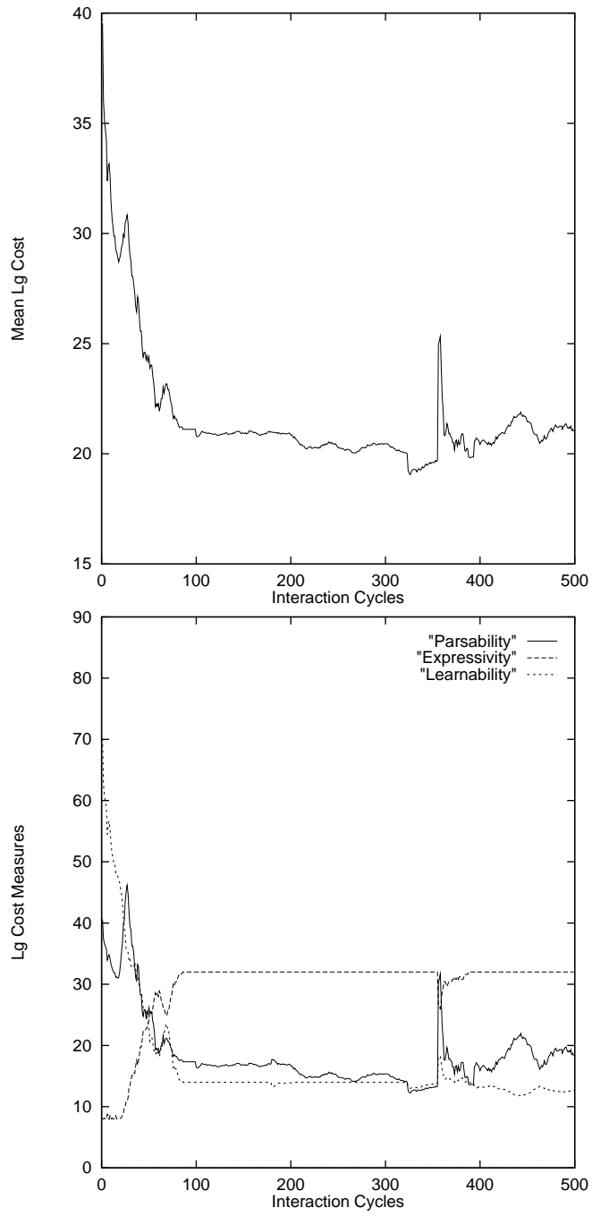
Figure 14: Language costs with random selection and migrations
