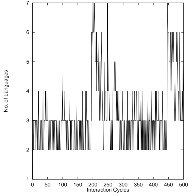
Figure 12: Number of languages in a typical run with migrations
