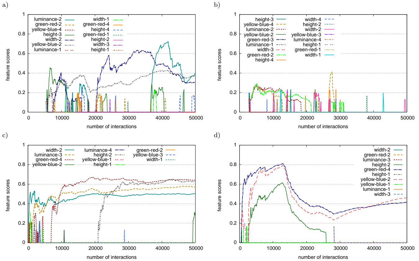
Figure 8. Examples of flexible word meanings. A population of 25 agents played 50000 language games. Each graph shows, for one particular word in the lexicon of agent 1, the strength of the association to different features. In order to keep the graphs readable, the agents have only access to a subset of the 10 sensory channels ( width , height , luminance , green-red , yellow-blue ).
