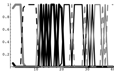
Figure 9: Discrimination-similarity game of a reinforcement learner with a non-uniform color distribution. The leftmost 10 chips (the “hot spot”) are chosen in 50% of the cases, see text. Parameters are n = 40 , m = 6 , L = 15 , k_{sim} = 4 . The frame is taken after about 10^5 runs.
