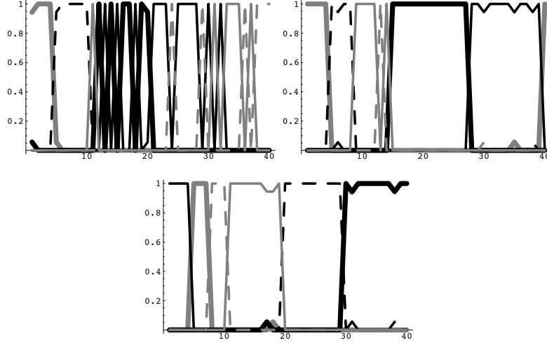
Figure 10: Discrimination-similarity game of a reinforcement learner with a non-uniform color distribution and non-constant k_{sim} . Parameters are n = 40 , m = 6 , L = 15 , k_{sim} varies between 2 for chips 1 – 10 and 6 for chips 11 – 40. The frame is taken after about 10^7 runs.
