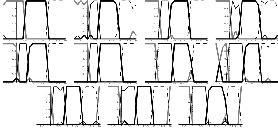
Figure 7: Several consecutive snapshots of the learning dynamics of a reinforcement learner playing the discrimination-similarity game. Here, we took L = 12 and k_{sim} = 3 . Initially, we have 3 dominant, deterministically assigned color categories, with a small perturbation introducing a small probability of the fourth color category for the first chip. The thick black, thick gray, thin black, and dashed lines correspond to the four color categories. There are 4000 rounds between consecutive snapshots.
