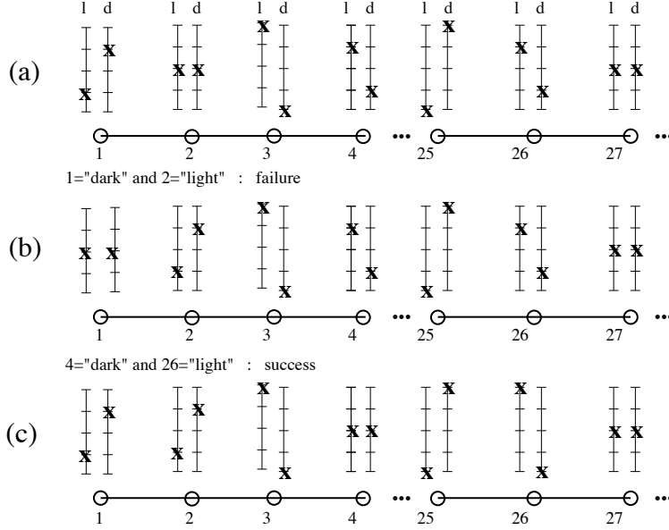
Figure 4: Two rounds of discrimination-similarity game with a reinforcement learner. Each color chip has two vertical lines or “ stacks ” for categories “light” and “dark” which successively track reinforcement updating. The current values of the stacks are denoted by the x . See text for the explanation of the updates performed by the learner.
