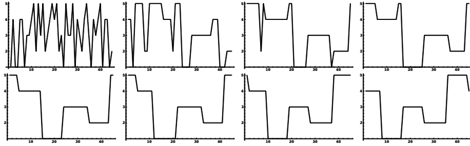
Figure 5: Several consecutive snapshots of the learning dynamics of a smoothing learner playing the discrimination game, starting from a random initial condition. The horizontal axes represent chips from 1 to n = 45 , and the graphs show the color assigned to each chip by the current categorization function. We took m = 5 categories and k_{sim} = 5 . There are 1000 rounds between consecutive snapshots. A leftward drift is noticeable, as seen by tracking the leftmost category (color 5), starting from the top right snapshot. In that snapshot, category 5 is assigned to chips 44, 45 and also chips 1–5. In the next few shots, category 5 moves to the left, reaching range 37 – 44 in the bottom right snapshot.
