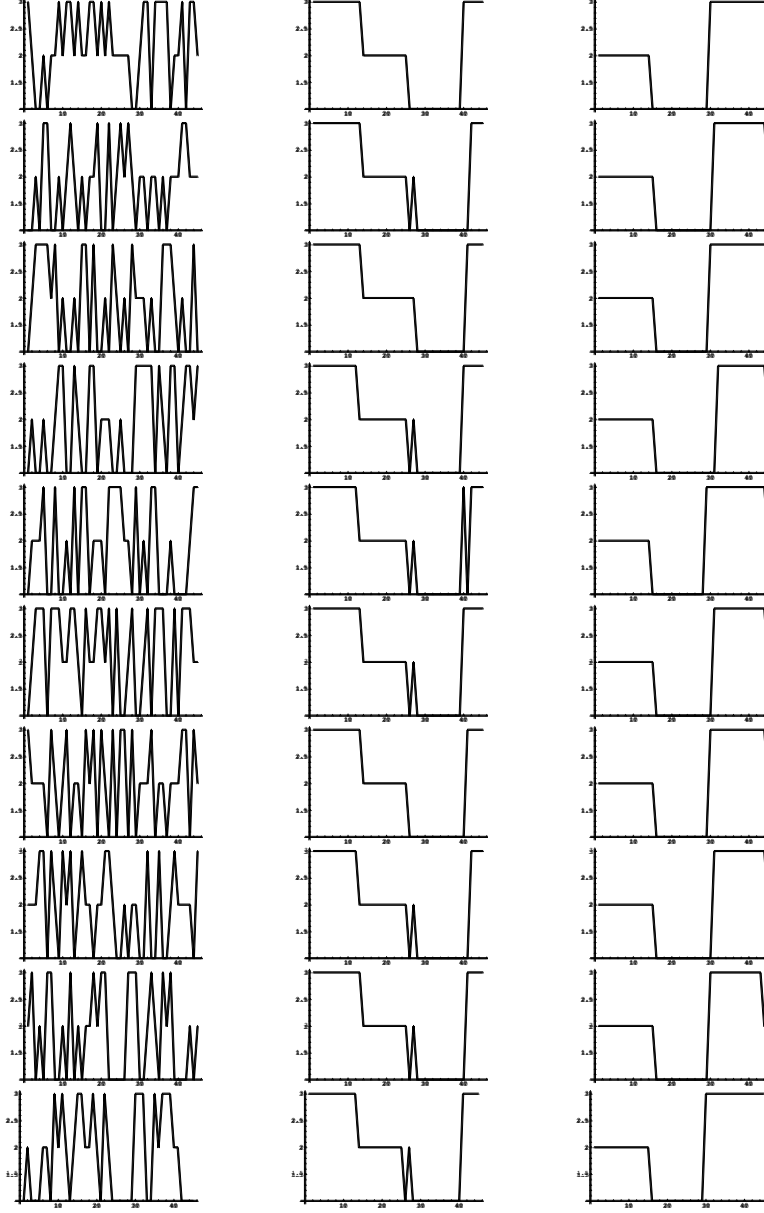
Figure 11: A population of smoothing learners playing the discrimination game, with N = 10 agents, n = 45 color chips, m = 3 and k_{sim} = 5 . The first column is the initial, random, color categorization of the ten players. The second column is the categorization of the players after 10,000 rounds of the game. The last column is the categorization 30,000 rounds later. For each chip (the horizontal axes) only one color category is shown: the one that the individual is most likely to use for this chip.
