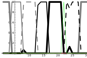
Figure 8: A snapshot of the reinforcement dynamics of discrimination-similarity game, with n = 30 chips, L = 16 , k_{sim} = 3 , and 8 color categories equally distributed initially. m_c = 6.1 in this case. This shot corresponds to about 10^6 iterations of the game.
